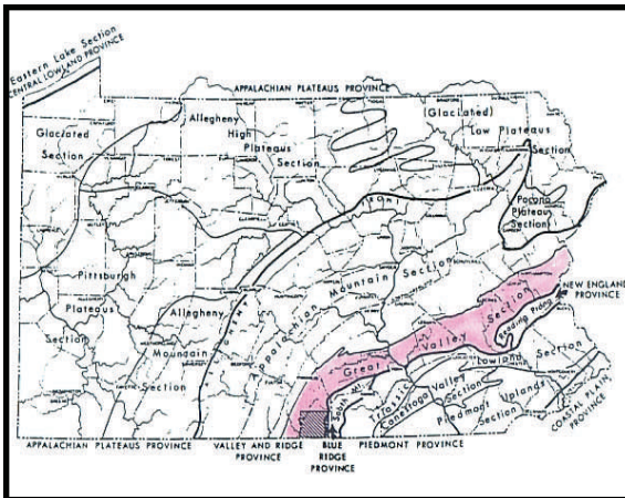
Physiographic Provinces of Pennsylvania (PA Geologic Survey)
