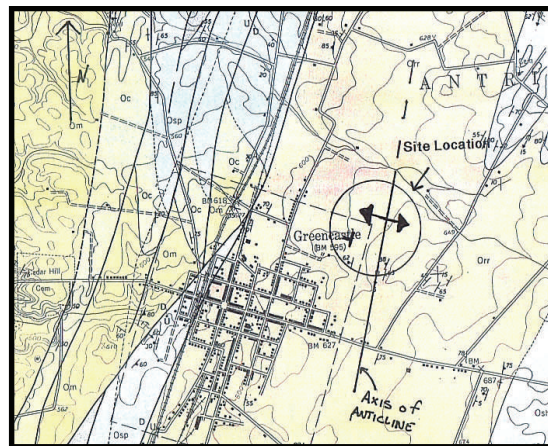
Geologic structure map of the Area of investigation
